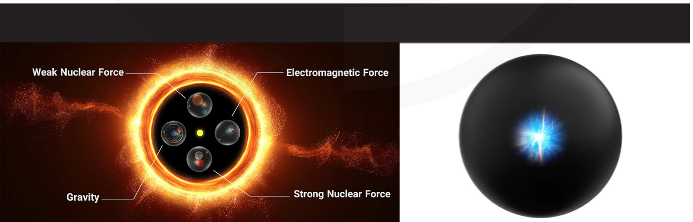
Figure 24: (Right image) Gravity is the only force present in the Cosmic Black Hole. (Left image) Presence of the four fundamental forces in a relative form in intra-cosmic black holes.
