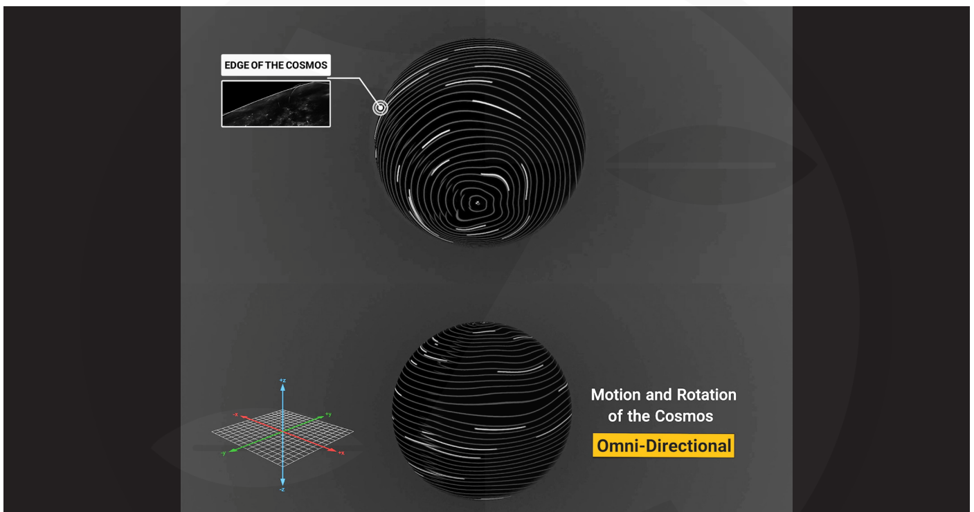
Figure 12: (Top image) The Terminal Edge of the Cosmos after the complete rebound of space mesh. (Bottom image) The rotation of the cosmos in the spherical cosmic model.
